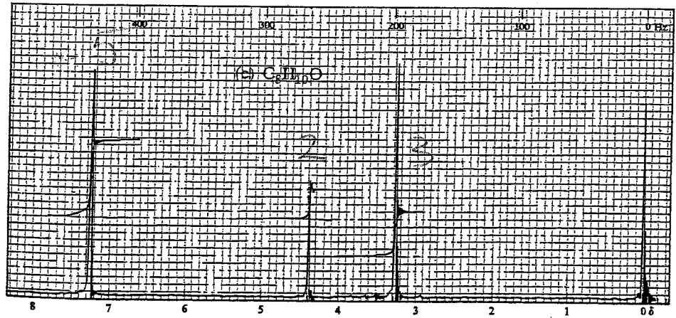
Figure 16.3. Nmr spectra for Problem 23, p. 546.
