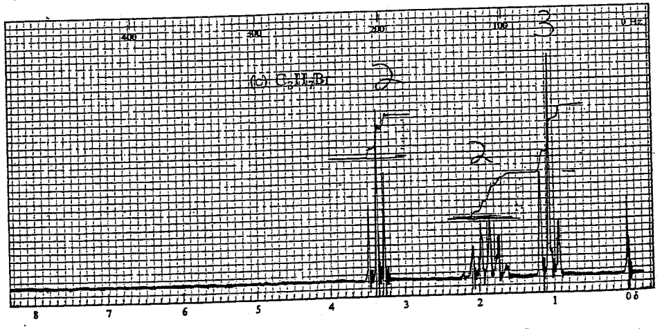
Figure 13.16. Nmr spectra for Problem 13.12, p. 435.
